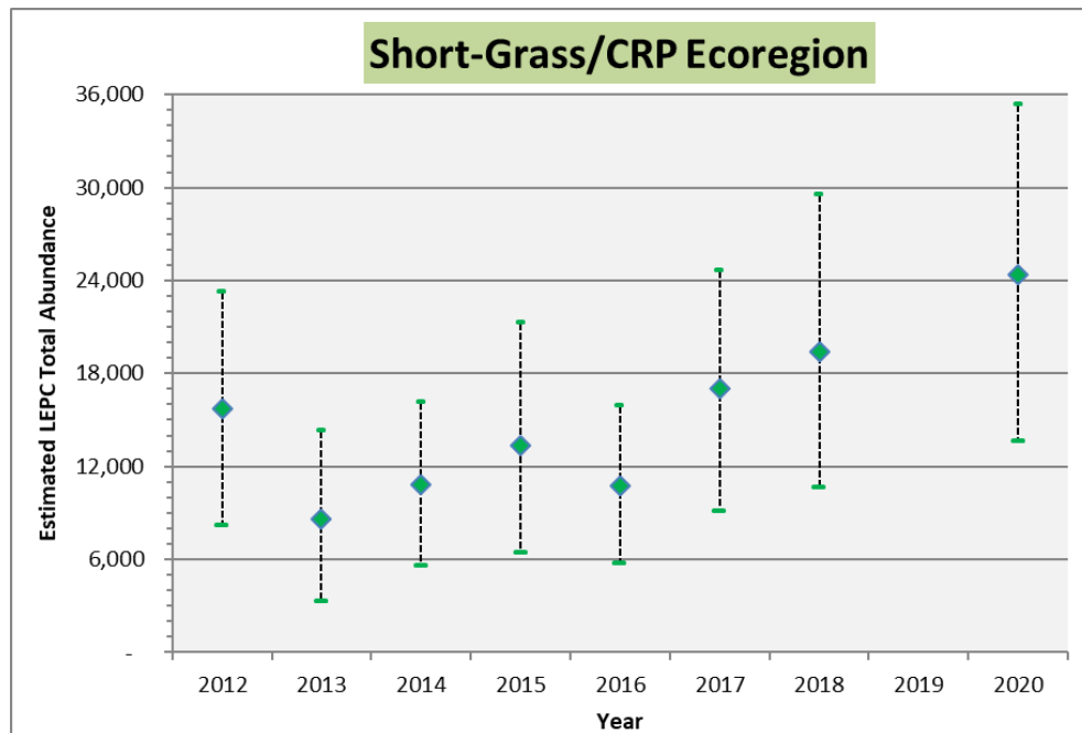
Figure 3.4 Annual estimates of breeding lesser prairie-chicken population sizes in the Short-Grass Prairie/CRP Mosaic Ecoregion from 2012 to 2020. Error bars are bootstrapped 90% confidence intervals. Graph reproduced from Nasman et al. (2020, Table 12, p. 21). Note that no aerial surveys were conducted in 2019.
