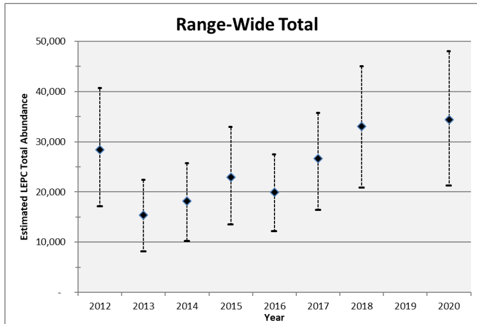
Figure 3.2 Annual estimates of total range-wide population size of lesser prairie-chicken from 2012–2020; bars represent the bootstrapped 90% confidence intervals. Graph generated from Nasman et al. (2020, Table 12, p. 21). Note there were no surveys in 2019.
