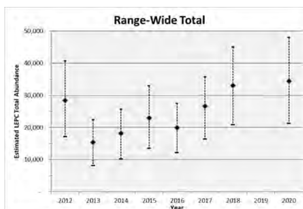
Figure ES.3 Annual estimates of total range-wide population size of lesser prairie-chicken from 2012–2020; bars represent the bootstrapped 90% confidence intervals. Graph generated from Nasman et al. (2020, Table 12, p. 21). Note there were no surveys in 2019.
