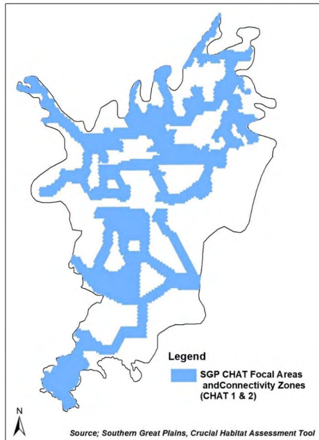
Figure B.12. Example, Mixed-Grass Prairie Ecoregion SGP CHAT Conservation Geographic Constraint.
