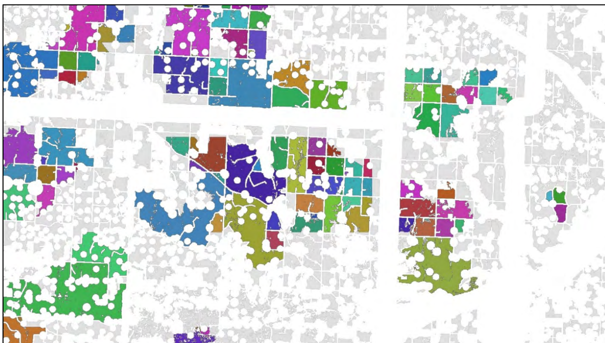
Figure B.13. Step 1. The different colors represent each individual un-impacted potential usable area polygon patch that intersected the 60% or greater neighborhood analysis threshold. The smallest separation between polygons is 140 meters.
