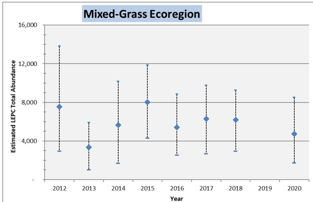
Figure 3.6 Annual estimates of breeding LEPC population sizes in the Mixed-Grass Prairie Ecoregion from 2012 to 2020. Error bars are bootstrapped 90% confidence intervals. Graph reproduced from Nasman et al. (2020, Table 12, p. 21). Note that no aerial surveys were conducted in 2019.
