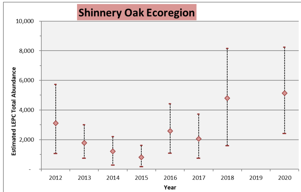
Figure 3.10 Annual estimates of breeding LEPC estimated population sizes in the Shinnery Oak Ecoregion in 2012 to 2020. Error bars are bootstrapped 90% confidence intervals. Graph reproduced from Nasman et al. (2020, Table 12, p. 21). Note that no aerial surveys were conducted in 2019.
