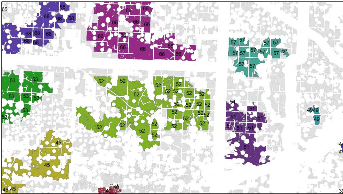
Figure B.15. Steps 4 and 5. The un-impacted potential usable area polygons are then dissolved by the Buff_ID field. All polygons within its group are now considered a block (shown as different colors in the map); one multi-part polygon (based on its intersection with the buffer layer polygons) with one acreage total equaling all its individual polygons in its group.
